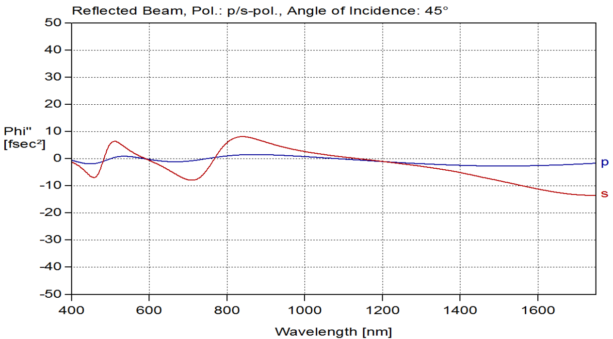
fig. 2 calculated GDD
