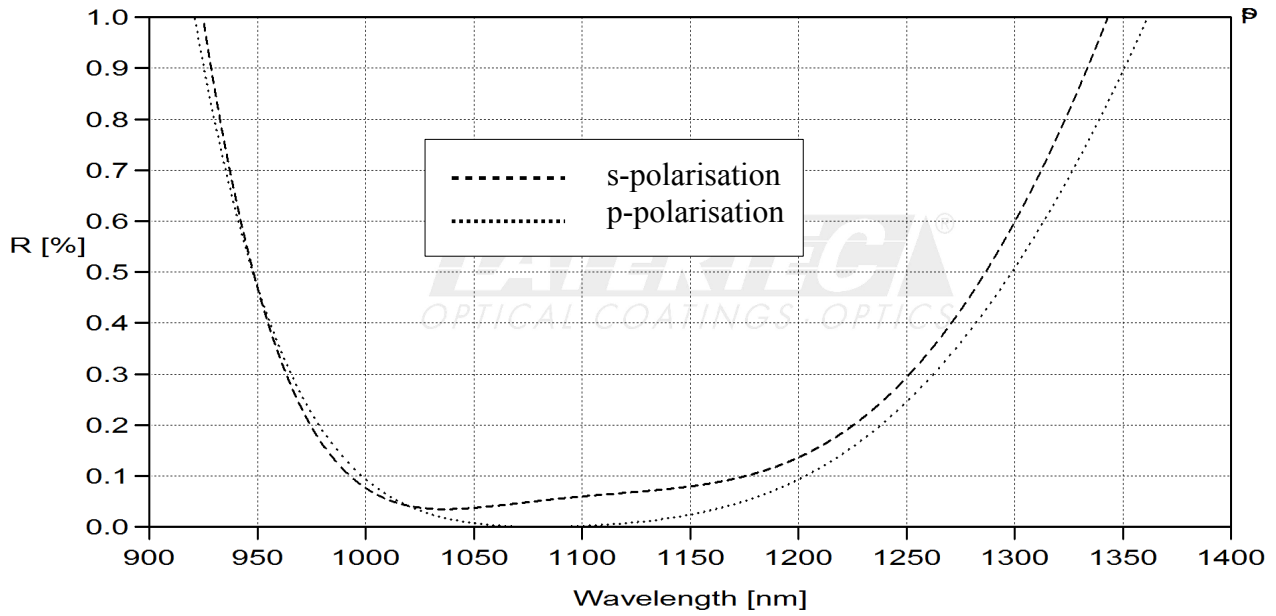
fig. 1 reflection AR 22.5°
